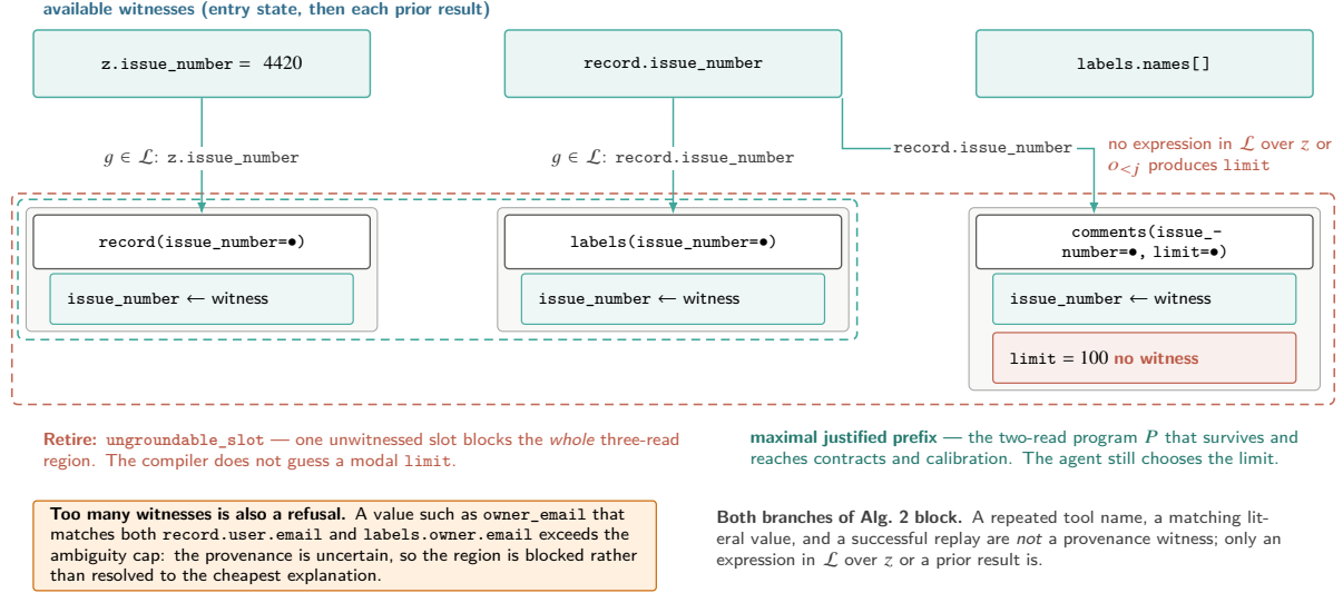
Figure 3: Equation (1) applied to the held-out issue-4420 record. Each argument slot needs an expression in \mathcal{L} over the entry state or a prior result; the green edges carry that expression, and the limit socket has no incoming edge at all. The diagram therefore asks a strictly harder question than recurrence: not “did this sequence repeat?” but “can every socket be wired from an allowed prior value?” One unwitnessed slot retires the whole three-read region, and a slot with too many witnesses does the same — both branches of Alg. 2 block rather than resolving to the cheapest available explanation. The ambiguity inset is illustrative; the wiring and the refusal are the executed compiler’s decision on that record.
