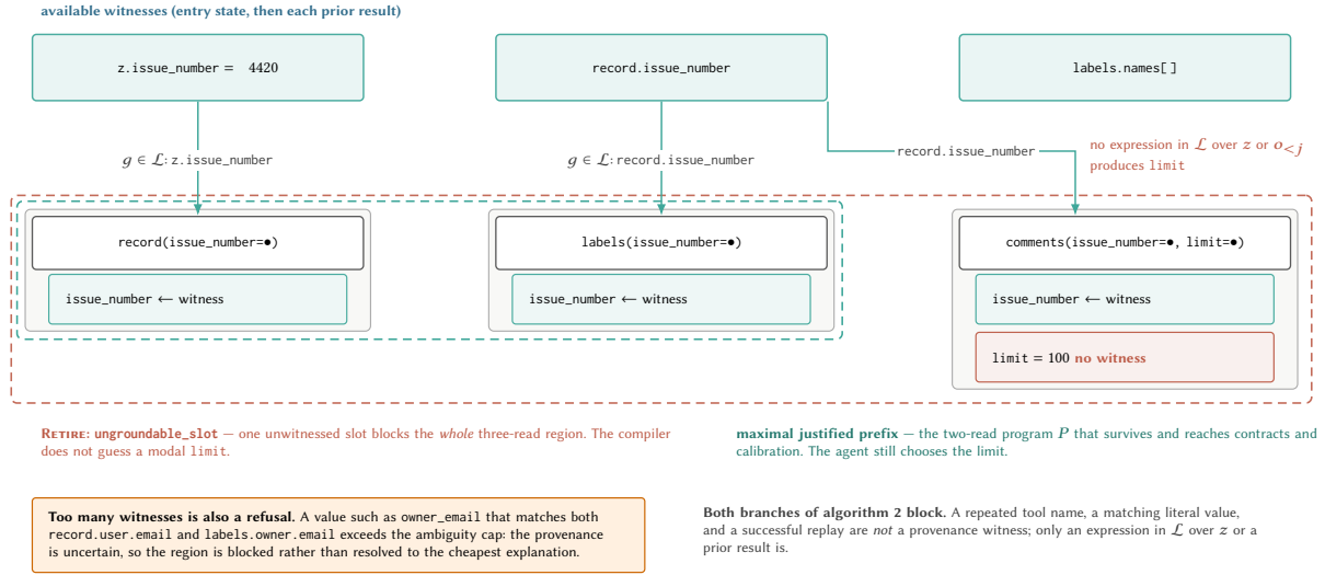
Figure 3: Equation (1) applied to the held-out issue-4420 record. Each argument slot needs an expression in \mathcal{L} over the entry state or a prior result; the green edges carry that expression, and the limit socket has no incoming edge at all. The diagram therefore asks a strictly harder question than recurrence: not “did this sequence repeat?” but “can every socket be wired from an allowed prior value?” One unwitnessed slot retires the whole three-read region, and a slot with too many witnesses does the same — both branches of algorithm 2 block rather than resolving to the cheapest available explanation. The ambiguity inset is illustrative; the wiring and the refusal are the executed compiler’s decision on that record.
