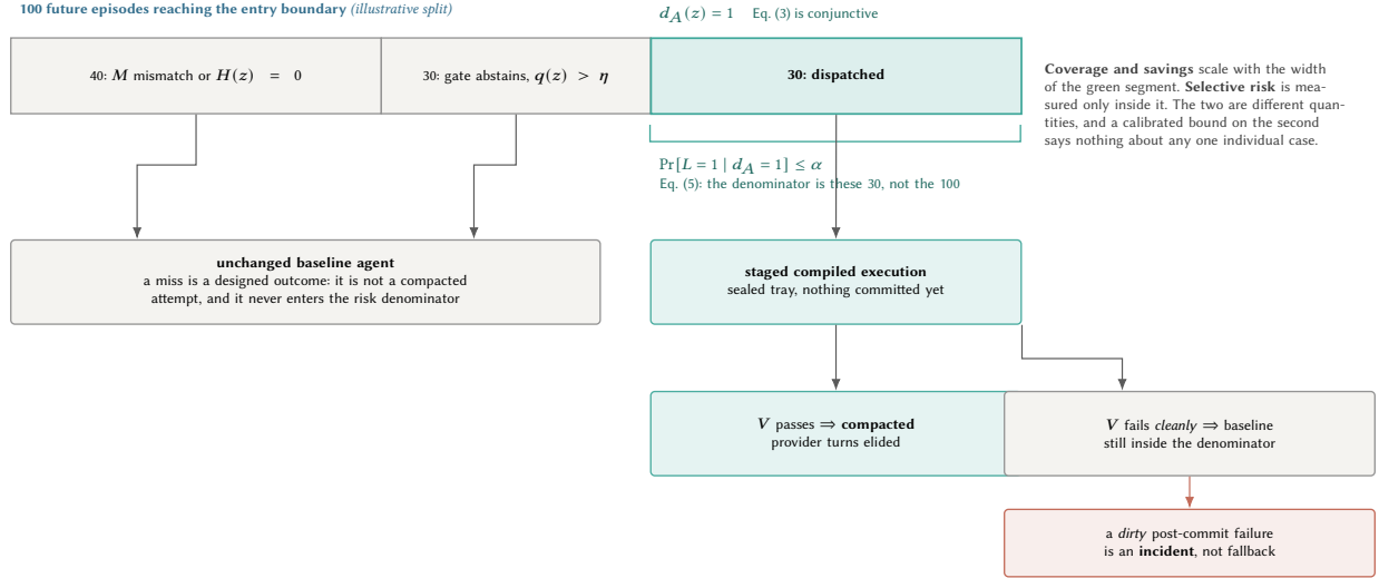
Figure 5: The population that Eqs. (3)–(5) quantify over, and the slice they condition on. Savings are earned across the dispatched segment, while selective risk is measured inside it: an episode that misses on the manifest, the guard, or the gate returns the baseline and never enters the denominator, so it is not a compacted failure. A staged failure caught before the commit line also returns the baseline, but it does stay in the denominator, and only a post-commit dirty failure is an incident. The 40/30/30 split is illustrative and is drawn only to separate the two quantities; no coverage rate is claimed here.
