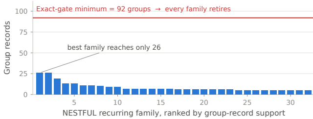
Figure 14: All NESTFUL families fall below the 92-group exact-gate requirement; the GitHub study was deliberately sized to reach it.
