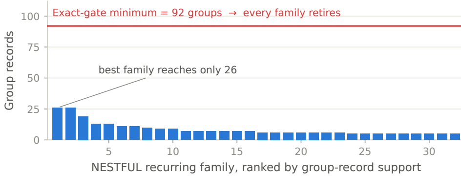
Figure 7: NESTFUL family supports against the 92-group requirement implied by eq. (7) at \alpha = 0.05 , \delta = 0.1 , |\Lambda| = 11 . The largest family reaches 26 groups, so every family retires at calibration even though provenance, synthesis, and replay all succeeded.
