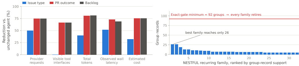
Figure 4: Left: reduction against the unchanged agent per family on the 30 held-out records each (the values of table 1; issue-type routing admits only a two-read prefix). Right: NESTFUL’s recurring families ranked by group-record support against the 92-group floor of eq. (7); the best reaches 26, so every family retires before calibration (section 5.3).
