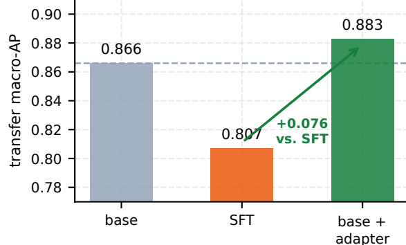
Q2 Composition recovers most of it, without retraining
