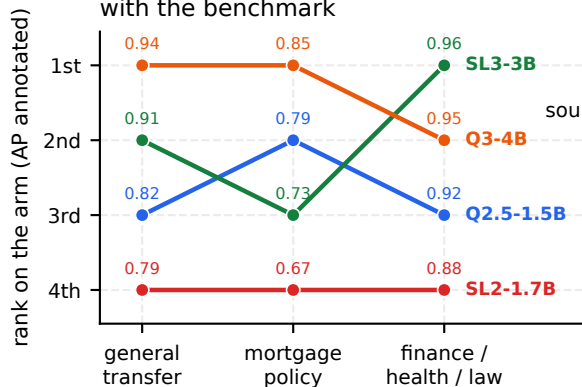
Q3 The top-ranked guard changes with the benchmark
