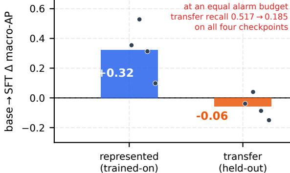
Q1 The benchmark gain does not transfer
