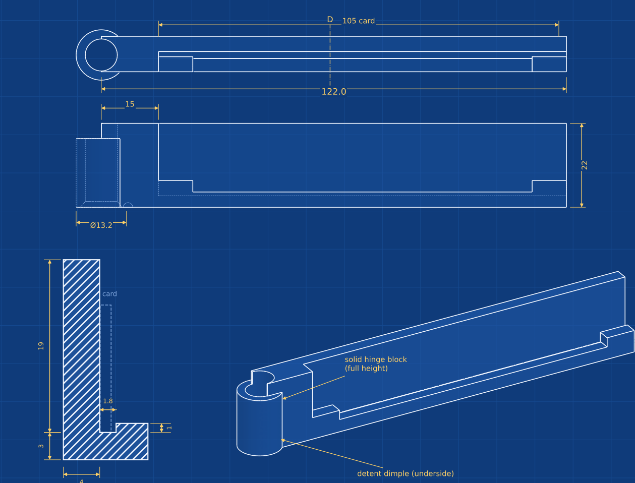
SECTION D-D (3:1) tall back wall 19, front lip 1, corner pads 4
