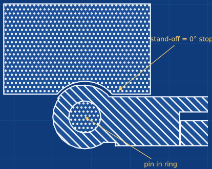
DETAIL B plan section through the hinge (2:1)
