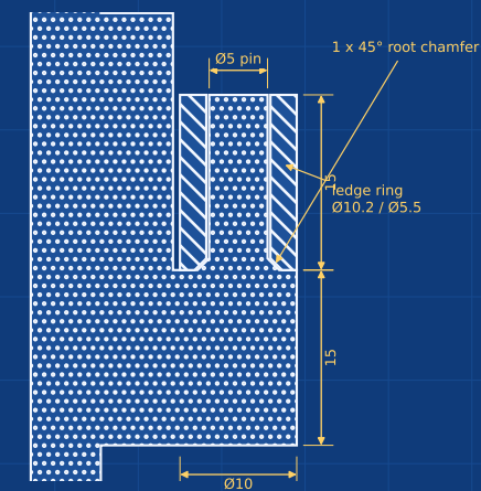
DETAIL A section on the pin axis (2:1) knuckle + pin from LiftOffHinge.stl; ledge ring sits on the knuckle
