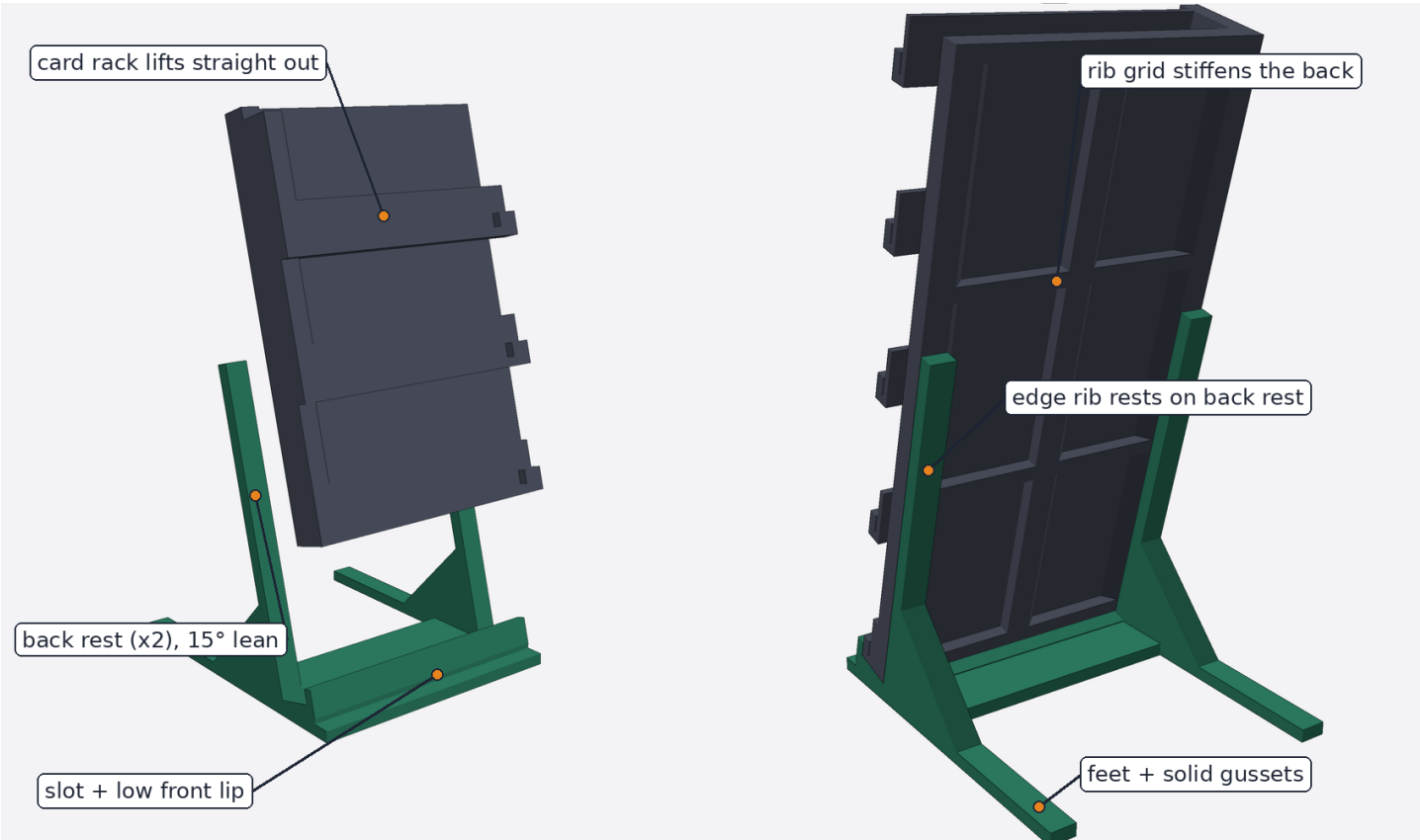
Left: the rack lifts straight out of the universal base. Right: the rib grid on the rack back sits on the base’s two back rests.
