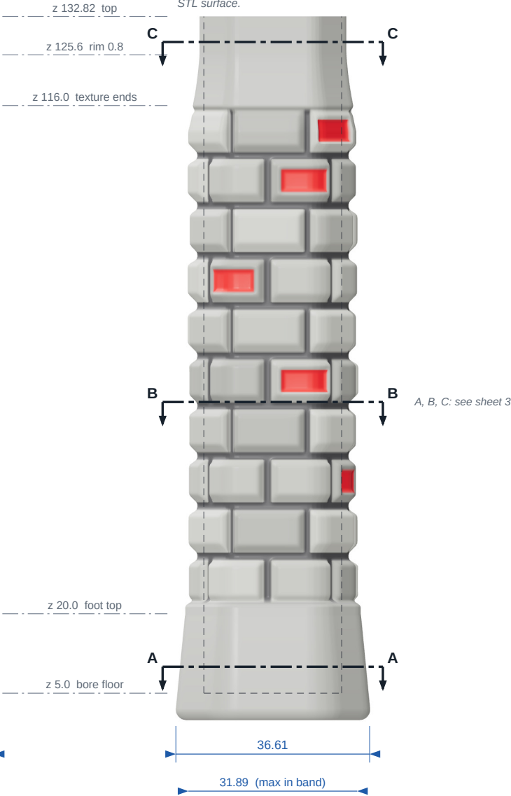
RIGHT VIEW (from +X)
