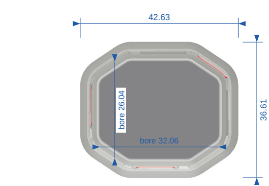
TOP VIEW (from +Z)
