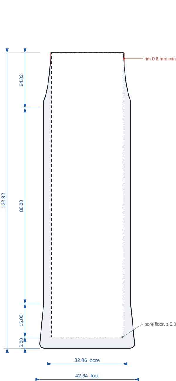
FRONT ELEVATION OF THE ENVELOPE (1 : 1)
