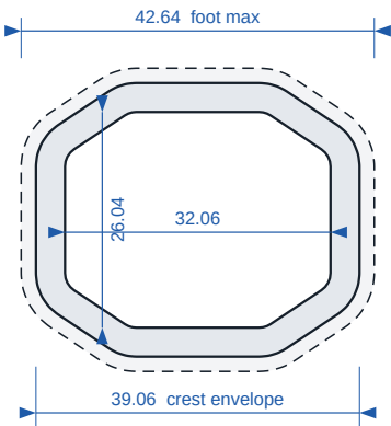
PLAN: BORE, CREST ENVELOPE, FOOT (1 : 1)
