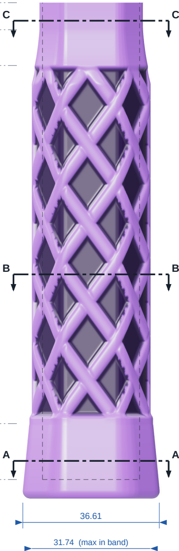
RIGHT VIEW (from +X)
