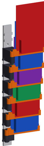
6-car kit on the 40 cm strip, closed: each row steps forward 7 mm, so every car and name stays in view.
