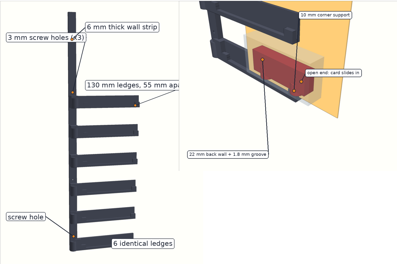
Left: the rack with its main features. Right: one ledge close up, with a card halfway in.
