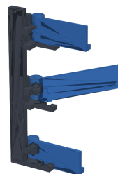
Print-in-place hinge: ledge 2 swung out 55°
