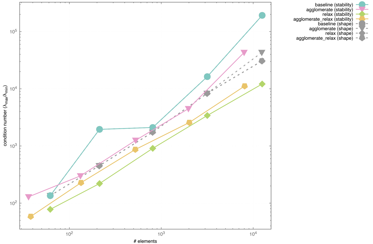
sorgente_40: conditioning -- stability (colour) vs shape (grey)
