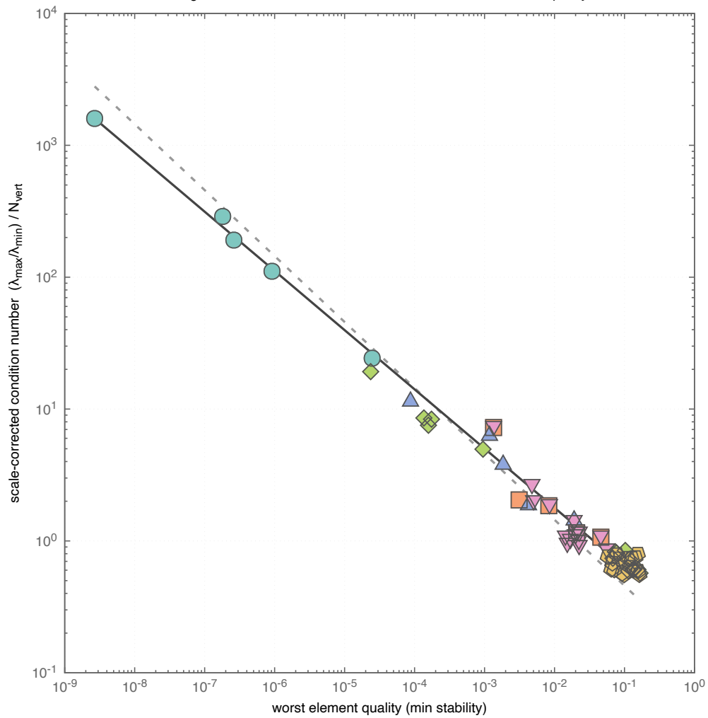
sorgente: scale-corrected condition number vs worst element quality
