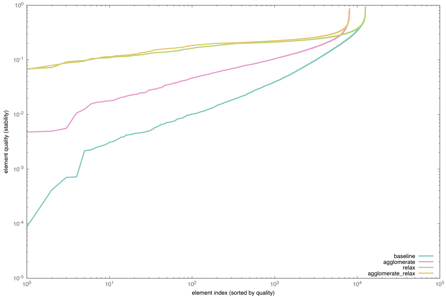
sorgente mesh5: quality vectors -- improving the Sorgente 40% mesh
