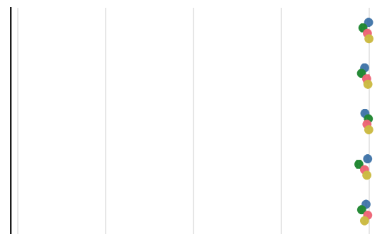
Preservation
