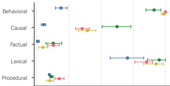
Boundedness
