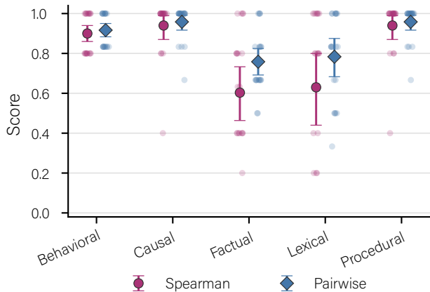
(B) Program-ranking fidelity by objective
