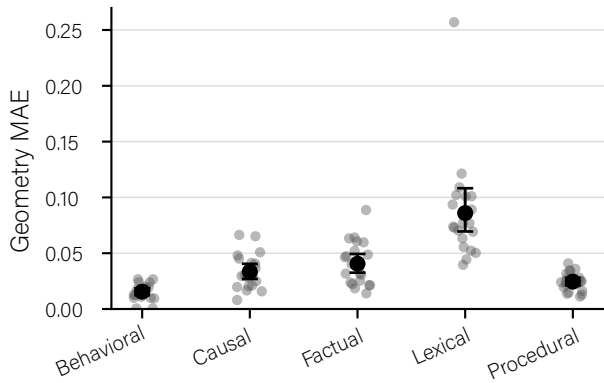
(A) Prediction error by objective
