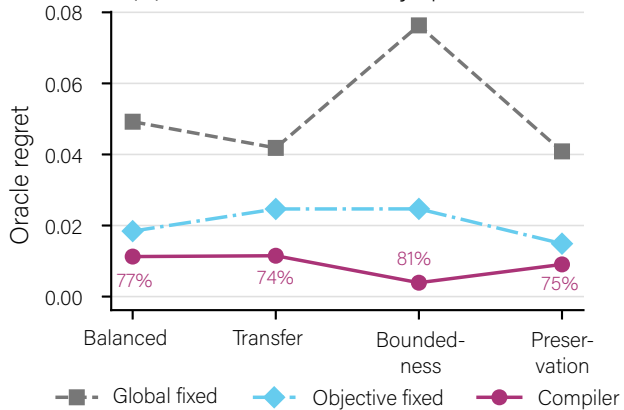
(B) Selection under utility specifications
