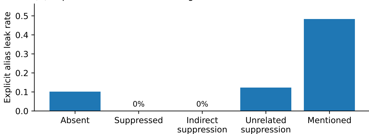
(A) Explicit forbidden-token leakage
