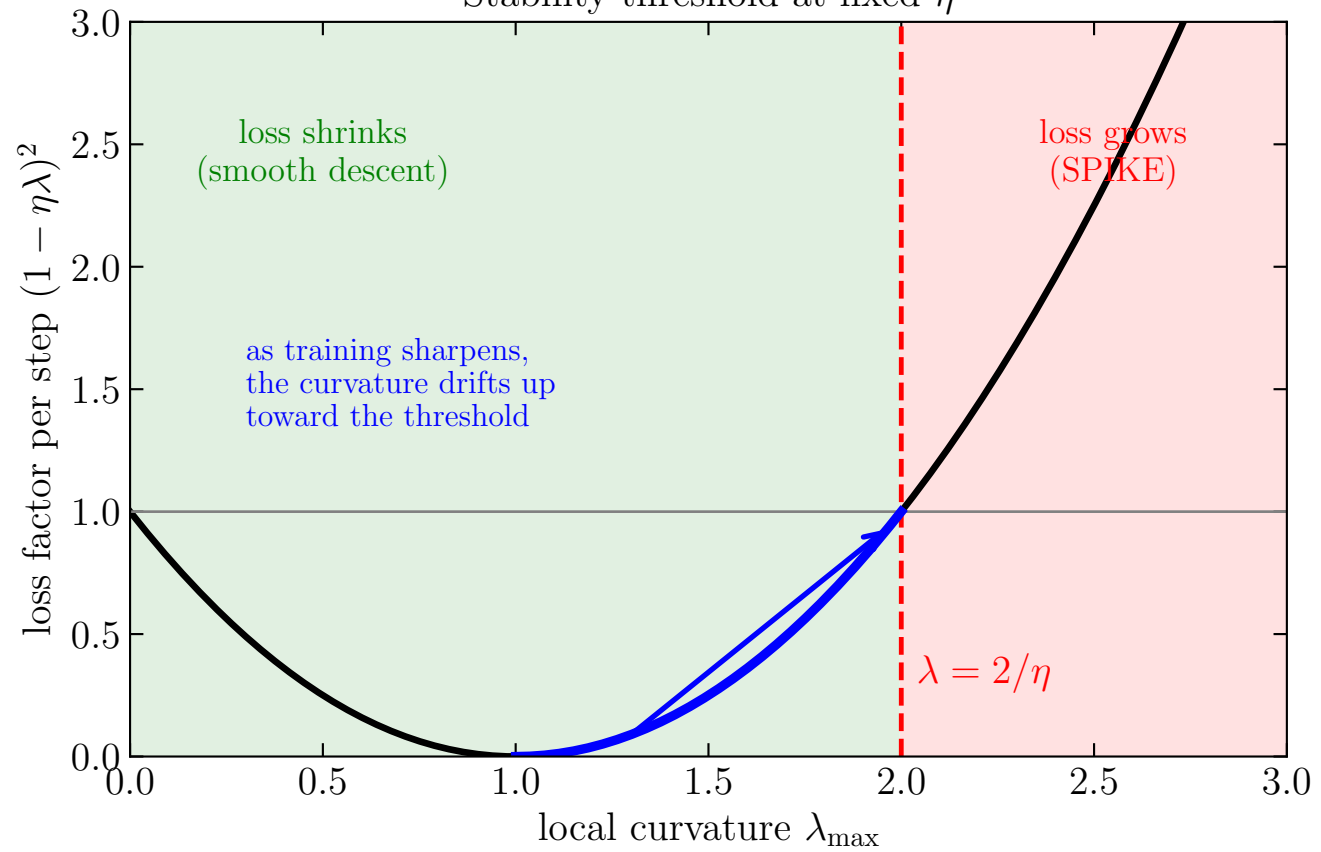
Stability threshold at fixed \eta
