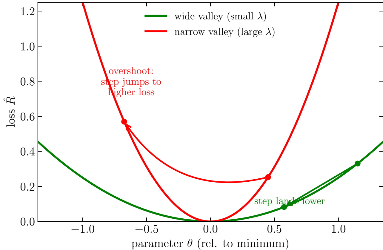
Same step size, two curvatures
