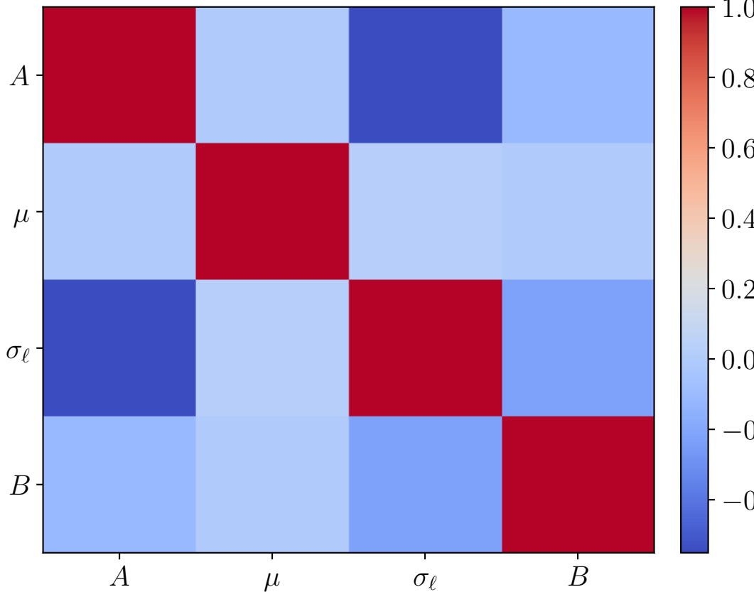
Estimated covariance from Hessian at \hat{\theta}_{\text{MLE}}
