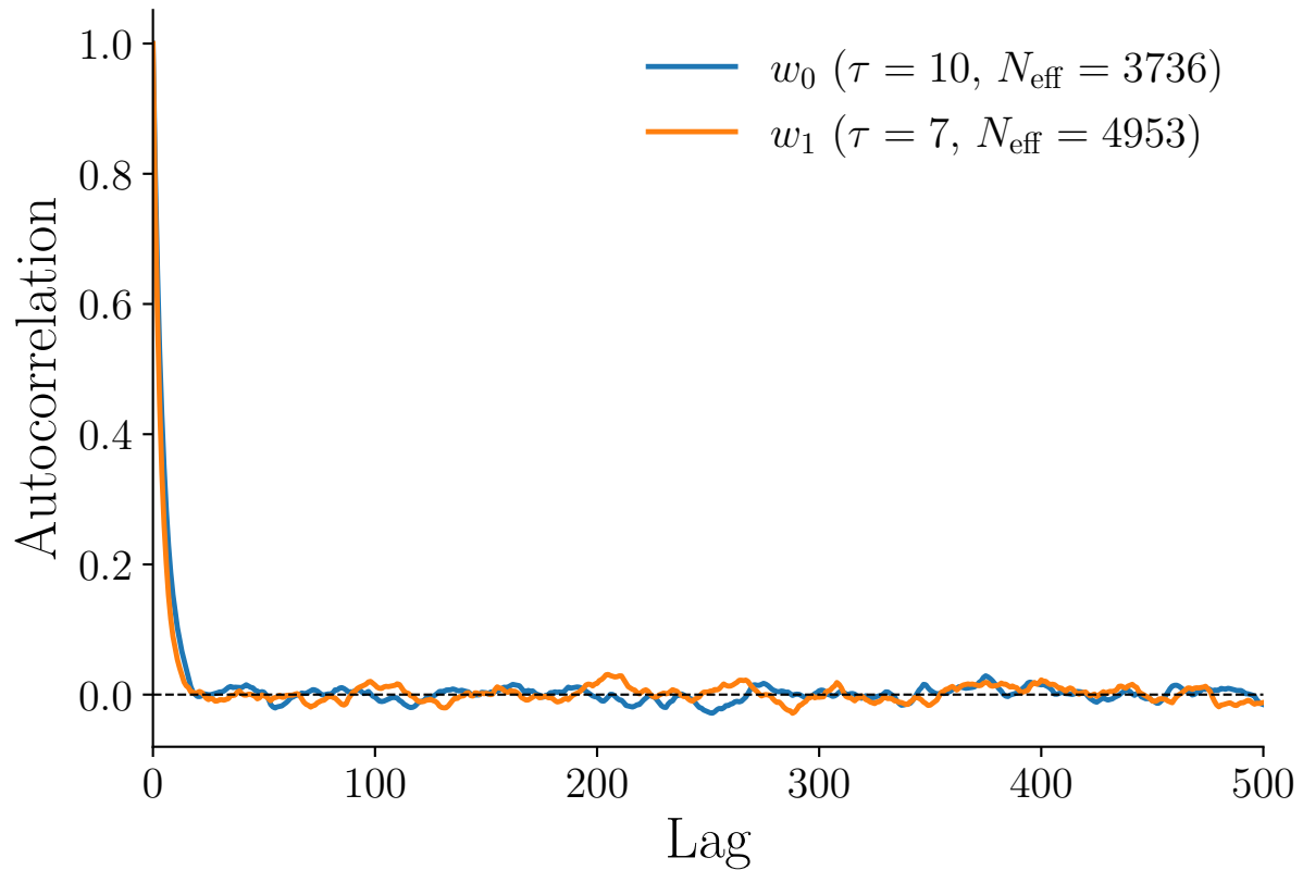
Autocorrelation function
