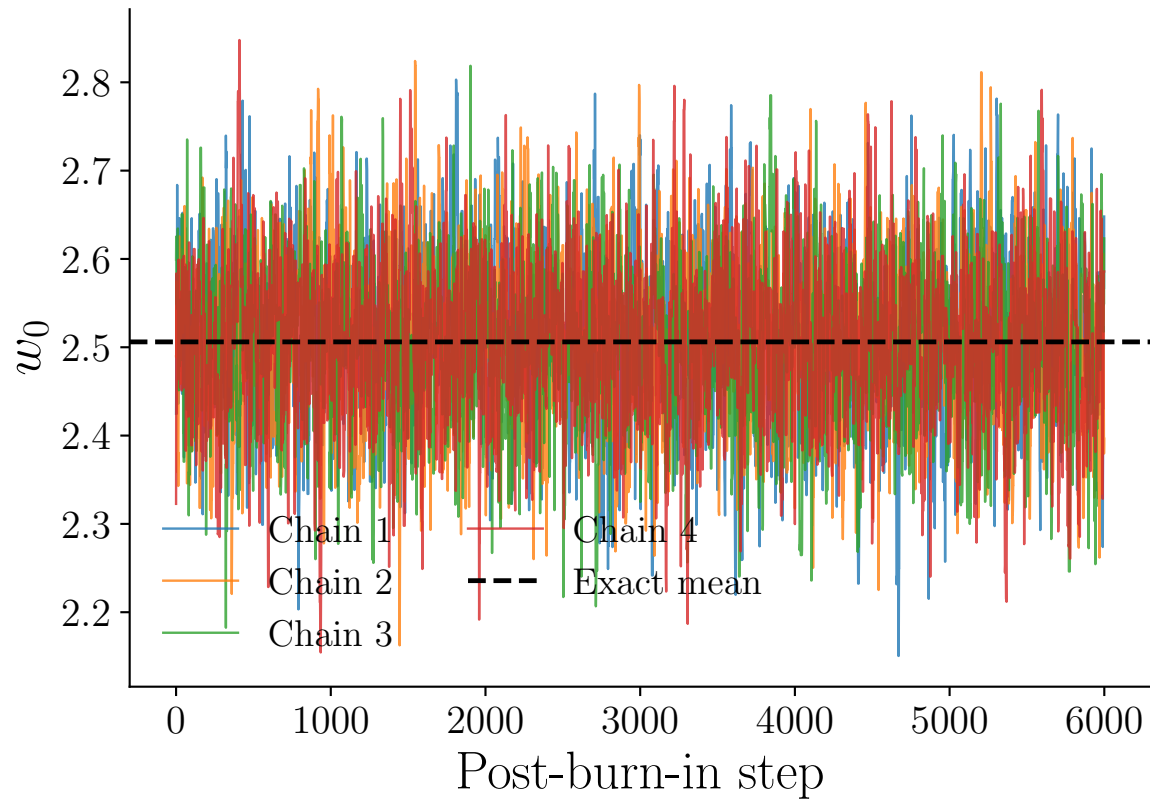
Gelman–Rubin \hat{R} = 1.0001
