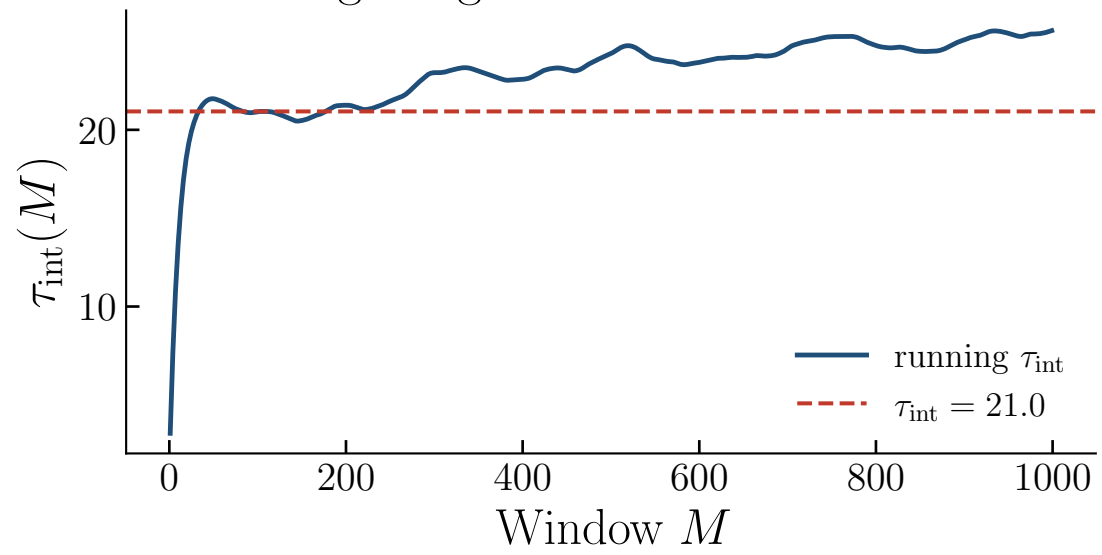
Running integrated autocorrelation time
