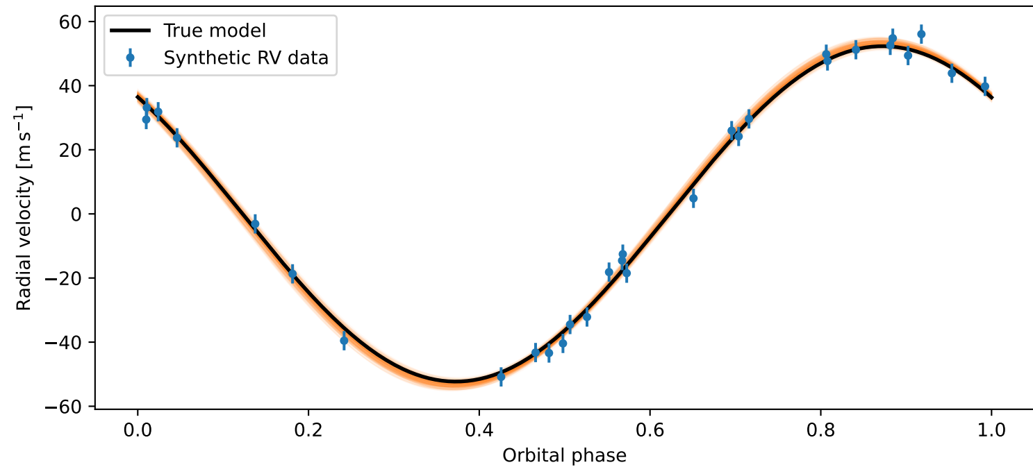
Phase-folded RV ( P_{\text{med}} = 4.233 d)
