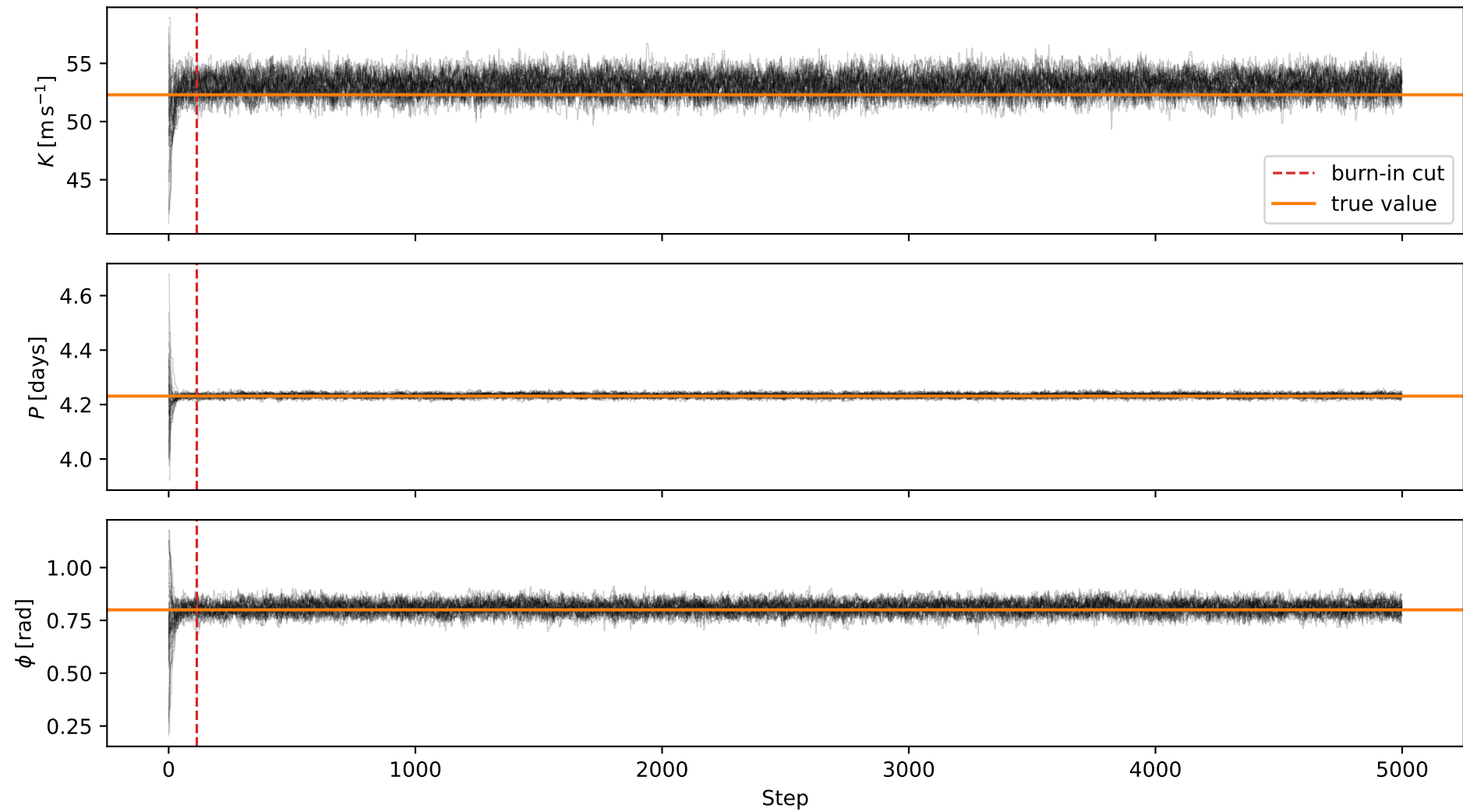
MCMC traces — exoplanet RV fit
