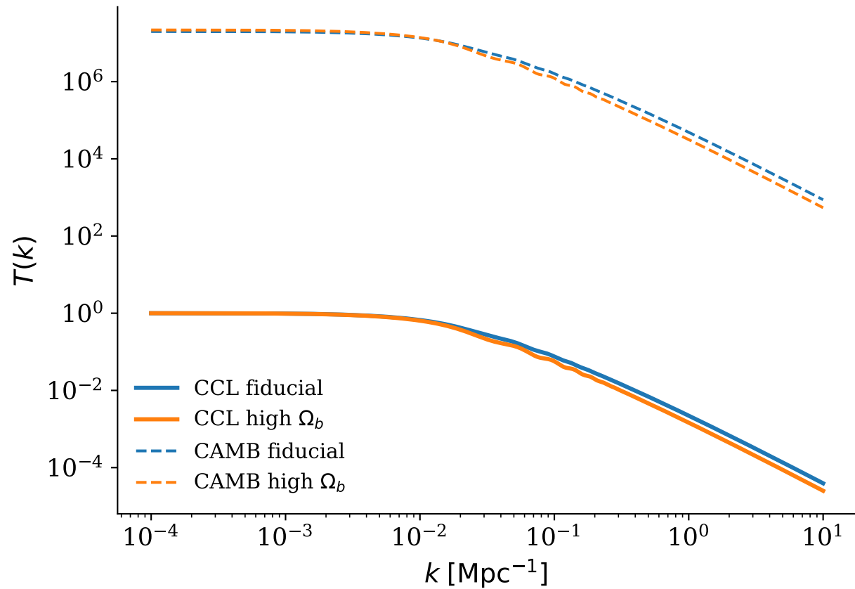
Linear matter transfer function
