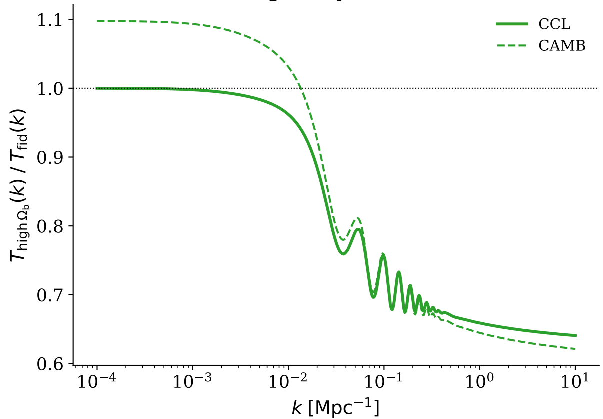
Ratio: high baryon vs. fiducial
