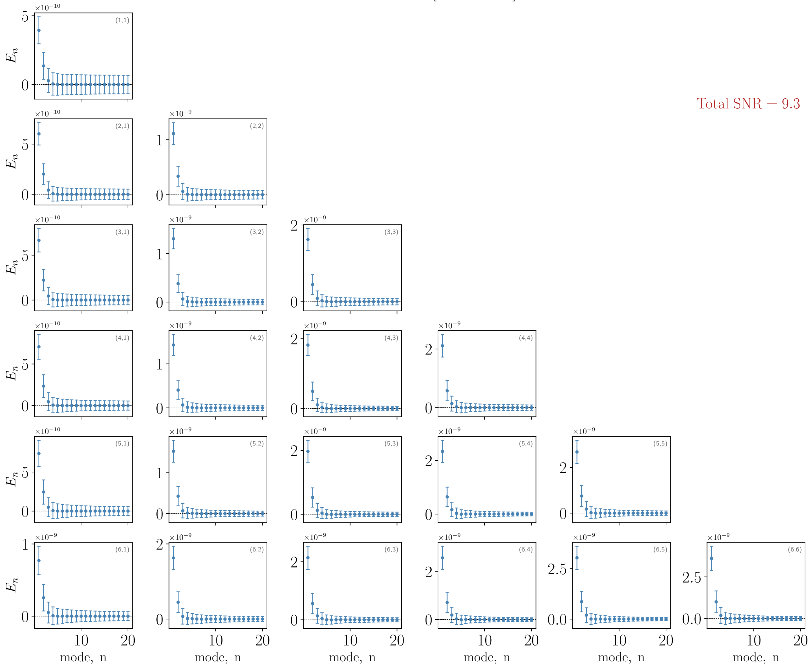
COSEBIs E-modes between [100.0, 300.0] arcmin
