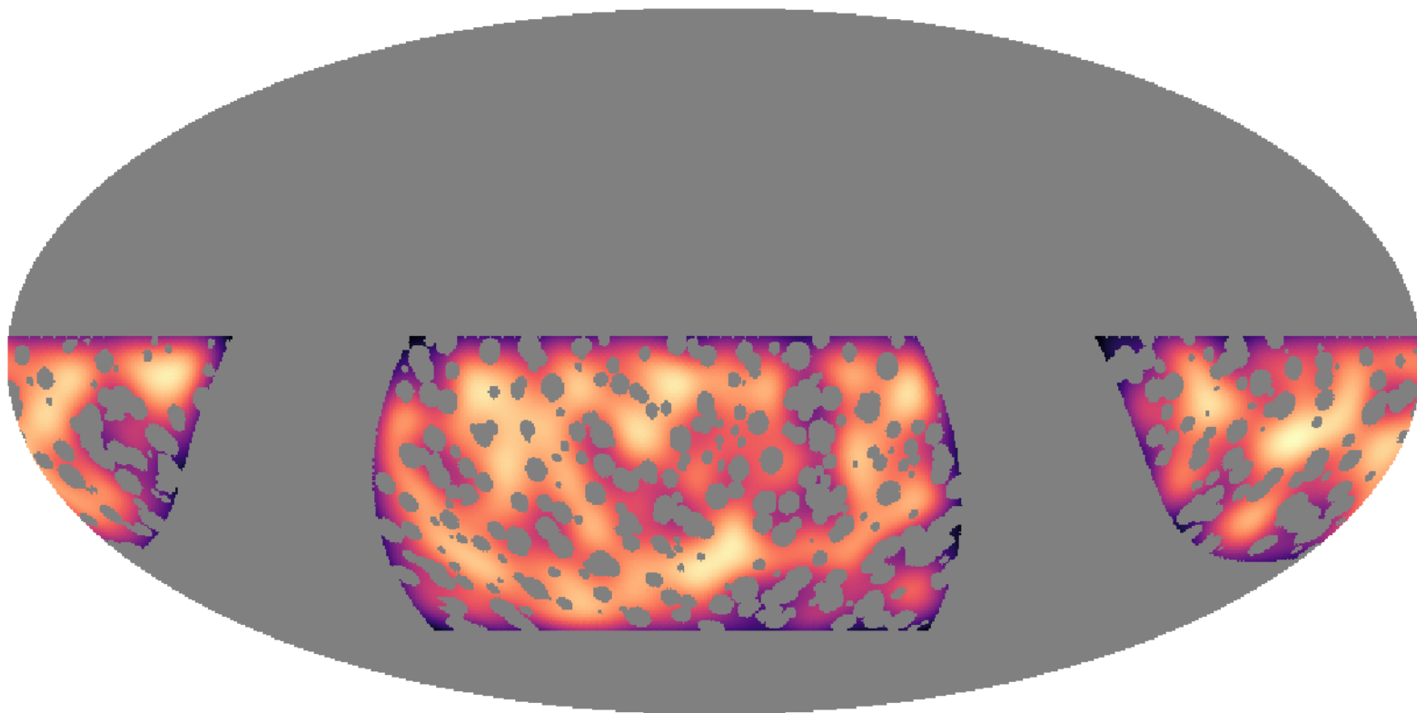
Local galaxy density
