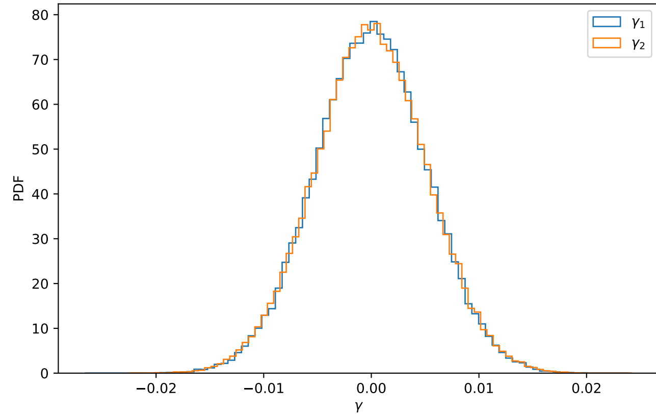
Shear distributions
