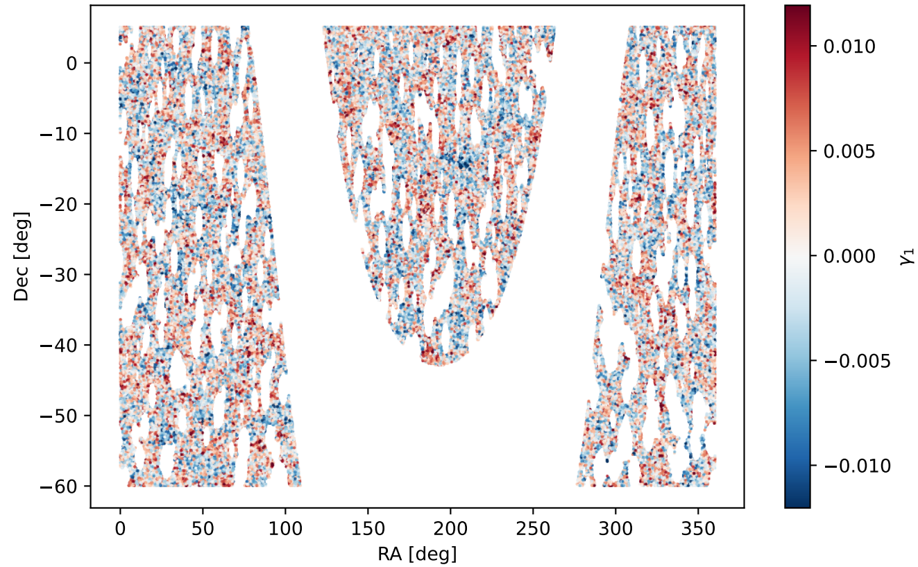
Sampled catalogue positions
