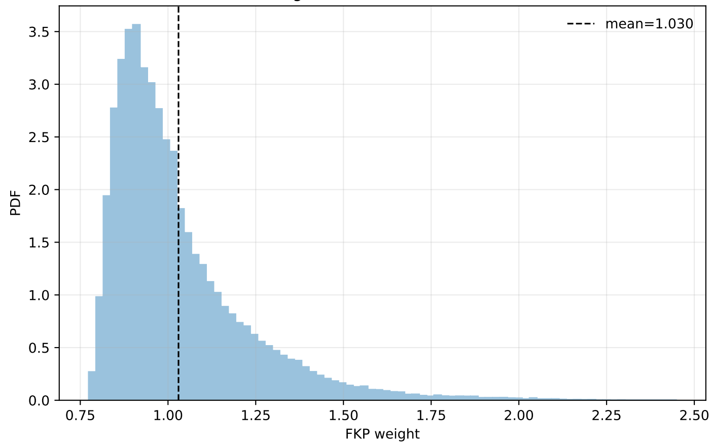
FKP weight distribution (realisation 1)
