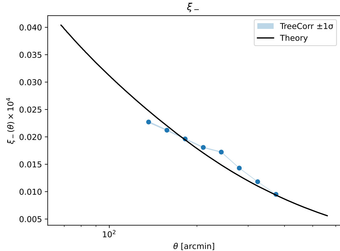
Shear two-point functions: measured vs theory (realisation 1)
