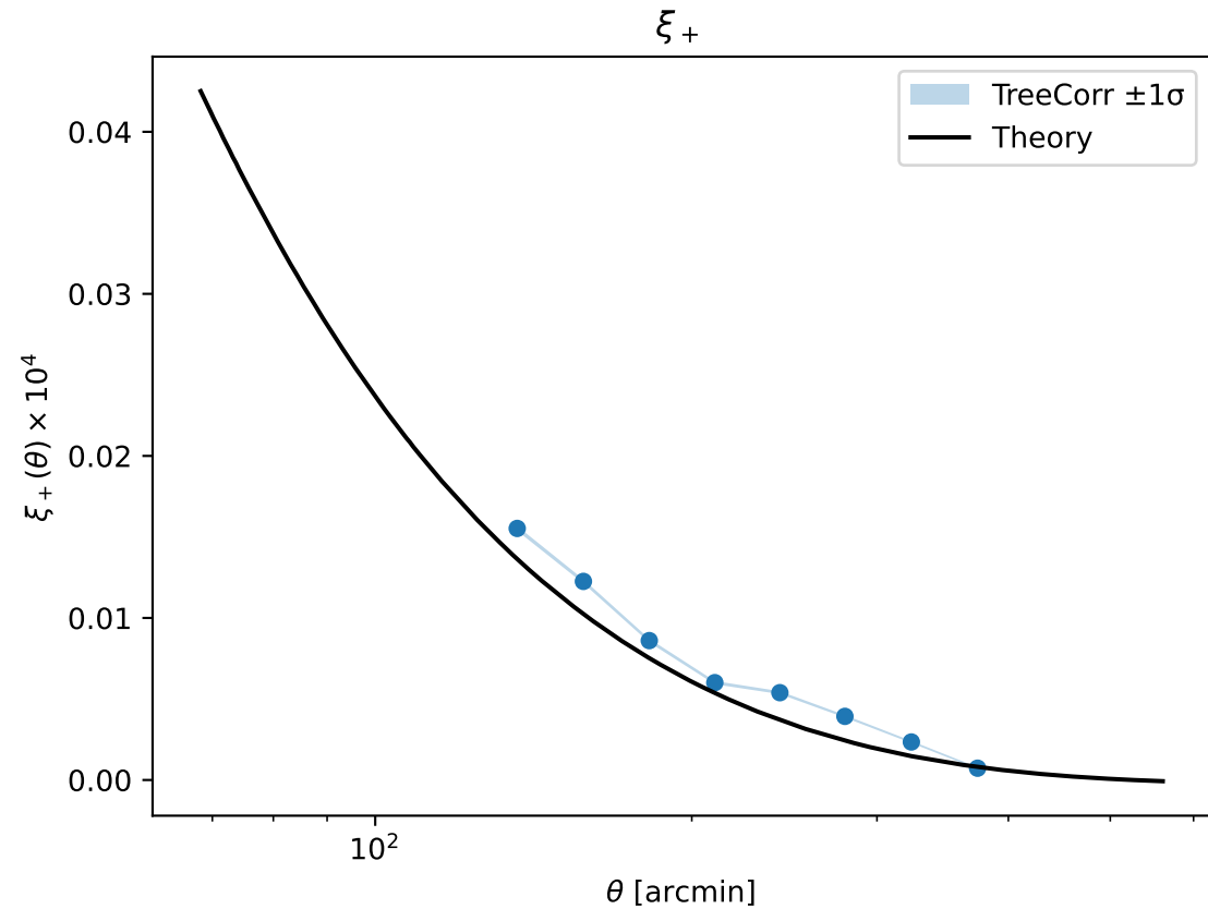
Shear two-point functions: measured vs theory (realisation 1)
