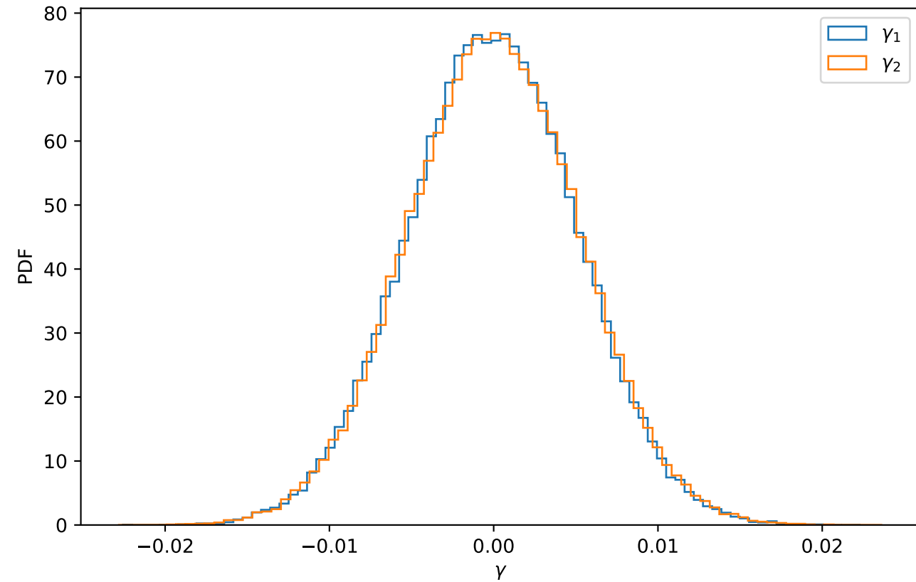
Shear distributions
