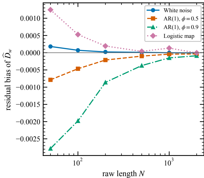
(a) Gap removes only short-range dependence
