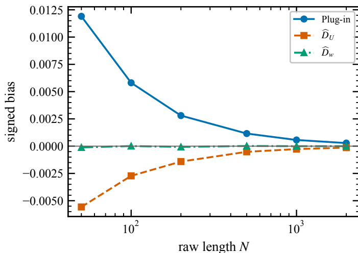
(c) IID white noise, m = 5
