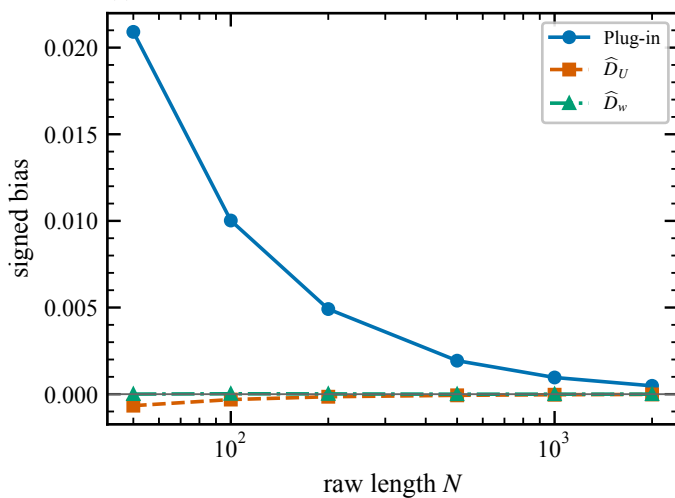
(c) IID white noise, m = 5
