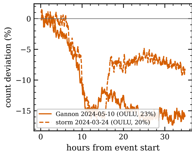
(c) Overlap-corrected structure vs event strength
