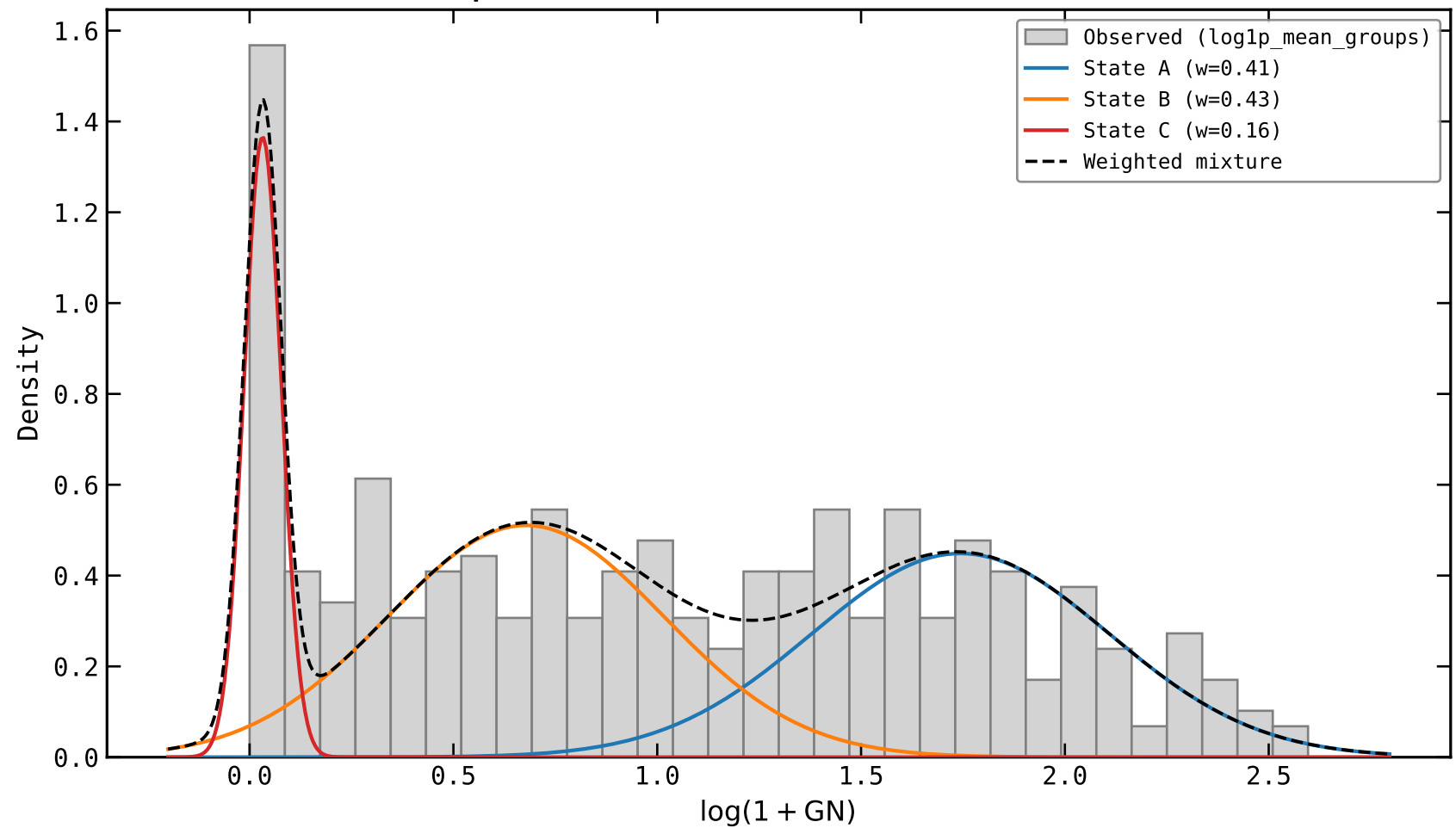
Fitted state-dependent Gaussian densities vs. observed distribution
