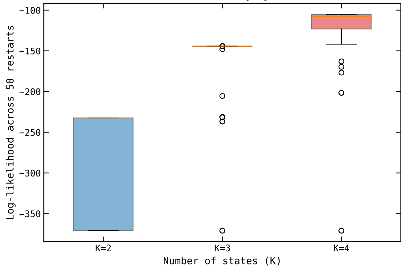
Restart-search stability by model size
