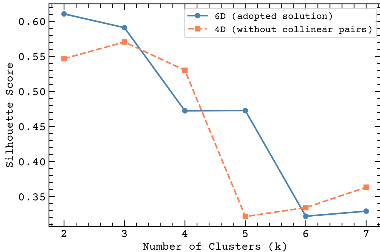
Silhouette Score: 6D vs 4D
