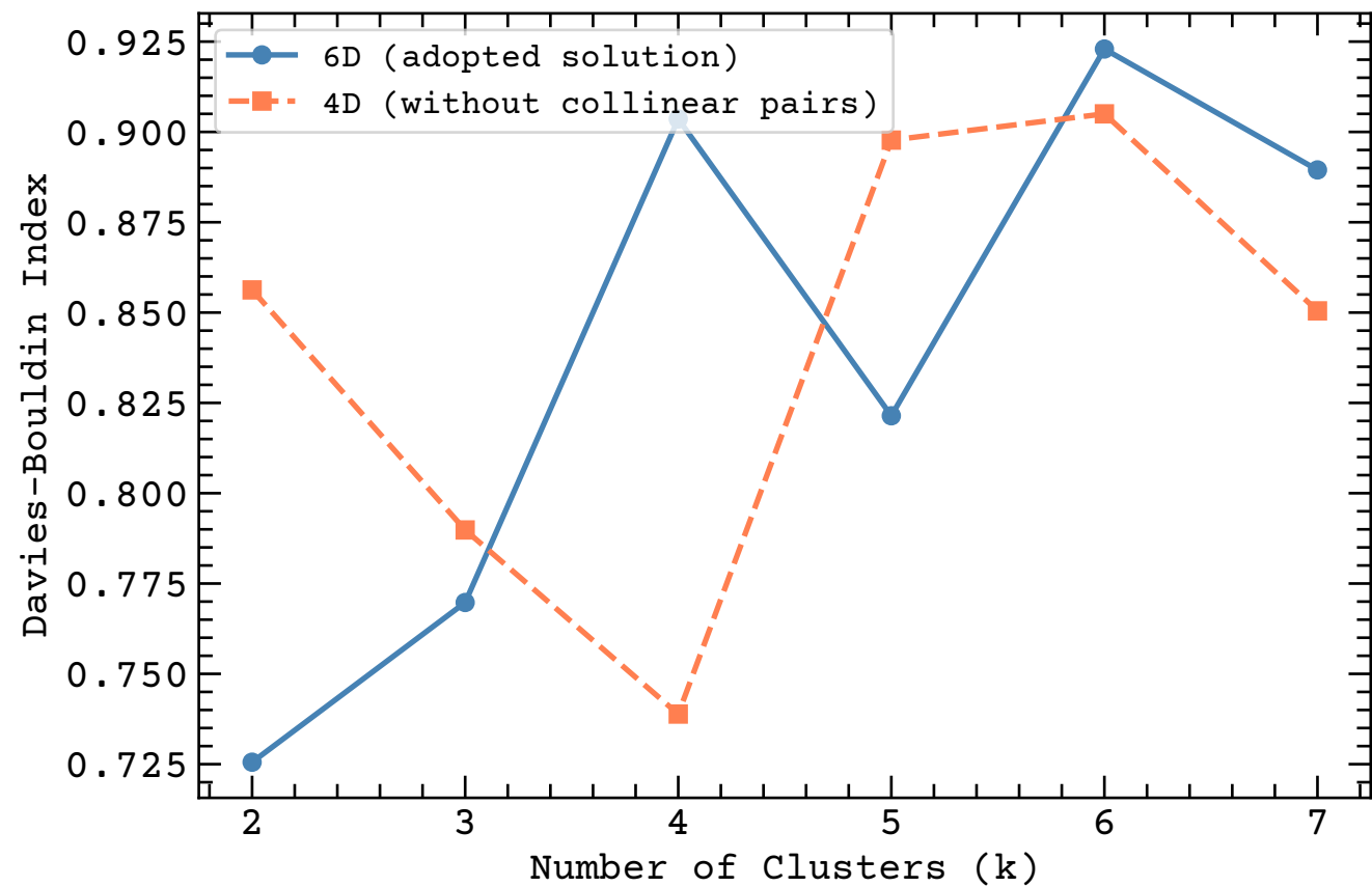
Davies-Bouldin Index: 6D vs 4D
