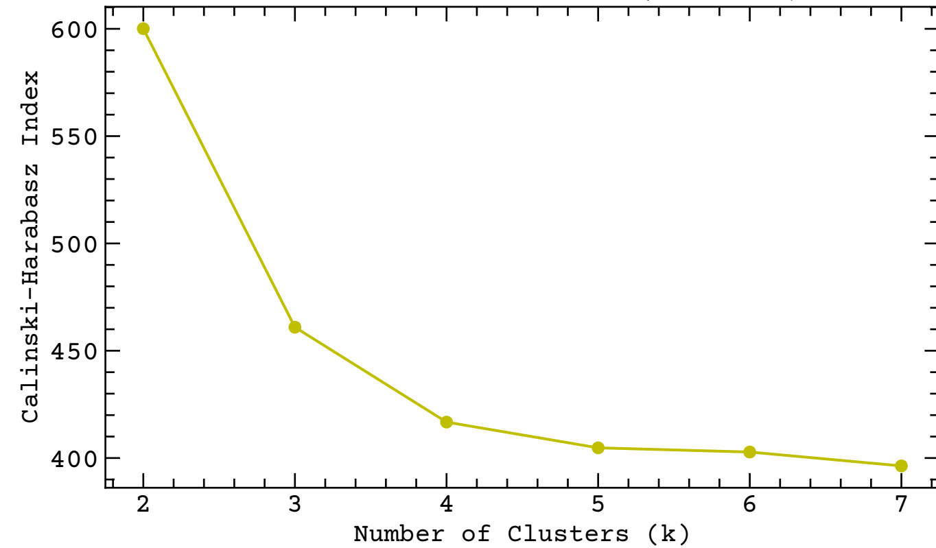
Calinski-Harabasz Index (Maximize)
