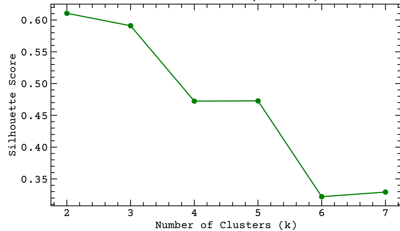
Silhouette Score (Maximize)
