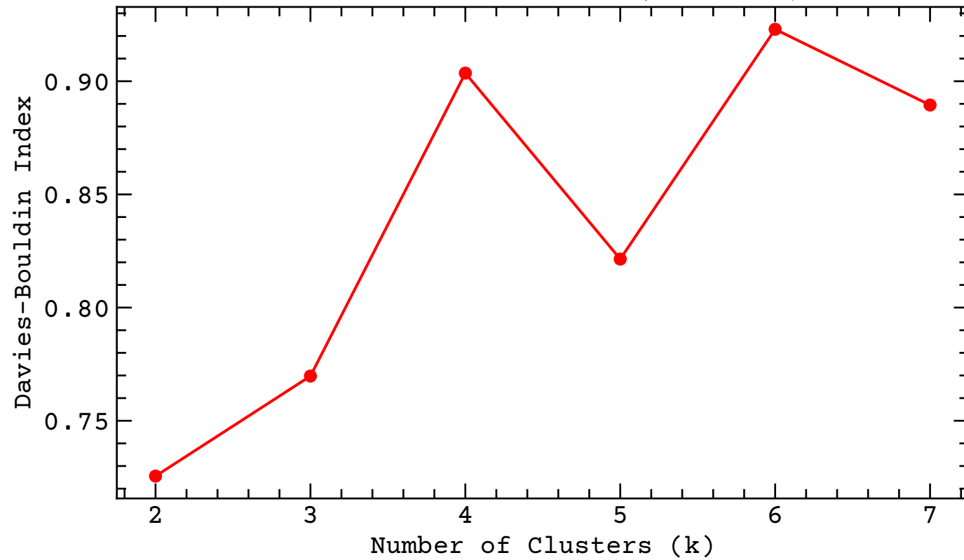
Davies-Bouldin Index (Minimize)
