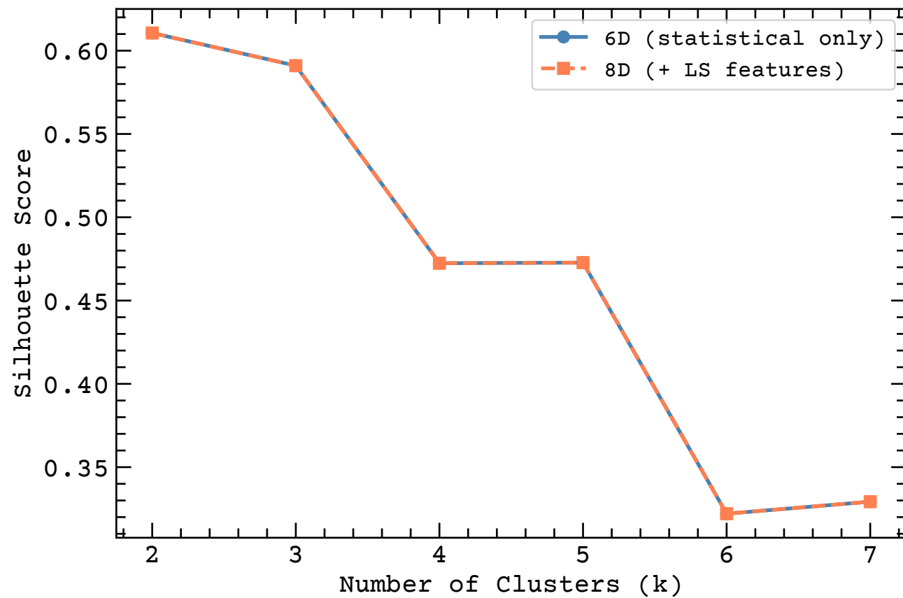
Silhouette Score: 6D vs 8D
