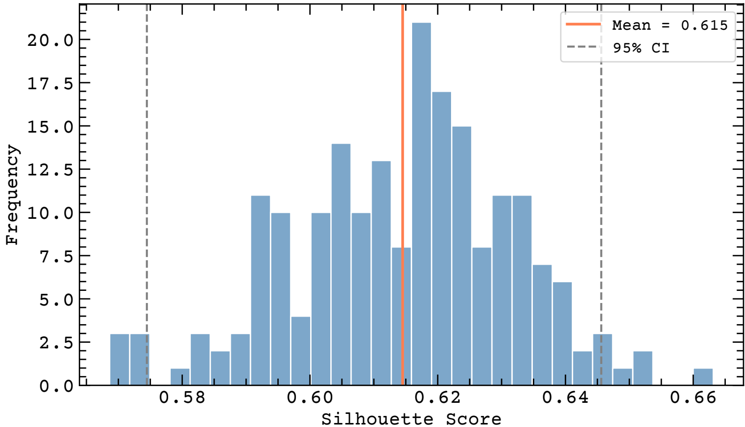
Bootstrap Distribution of Silhouette Score (k=2, n=200)
