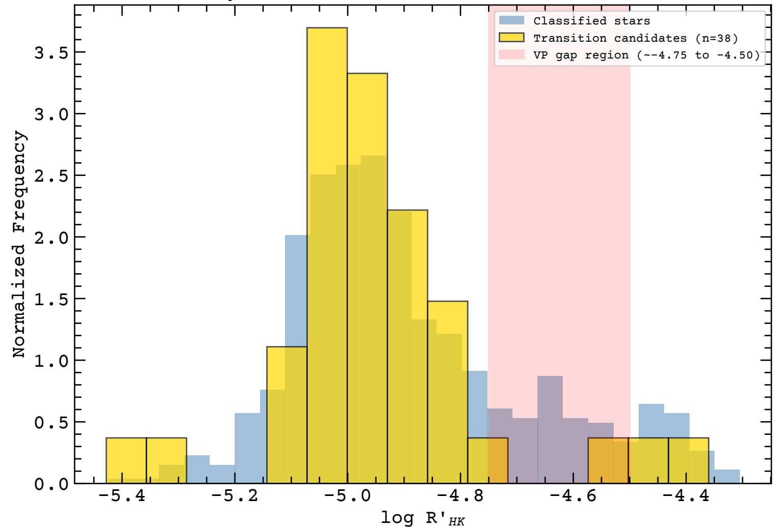
Activity Level: Transition vs Classified Stars
