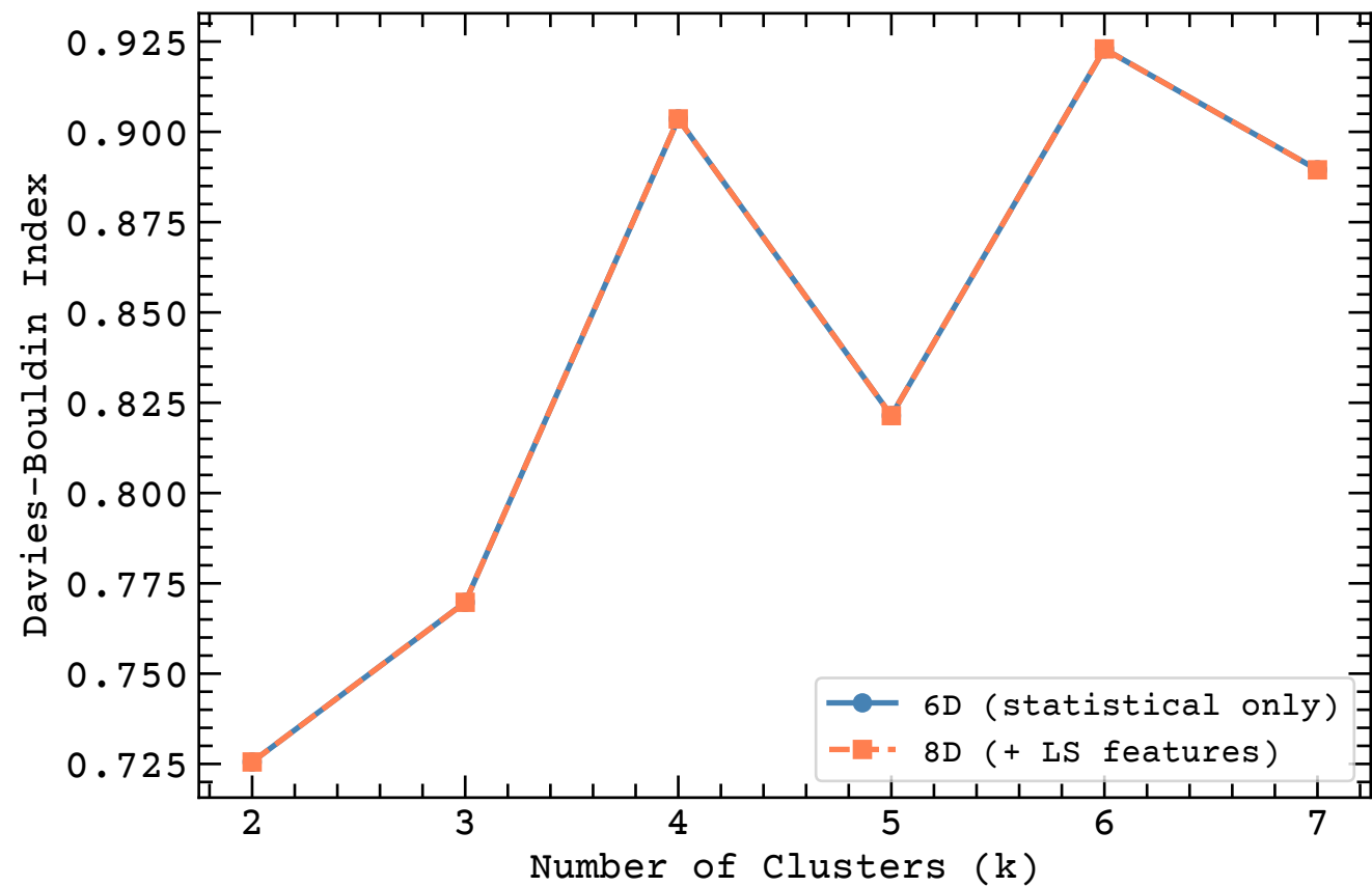
Davies-Bouldin Index: 6D vs 8D
