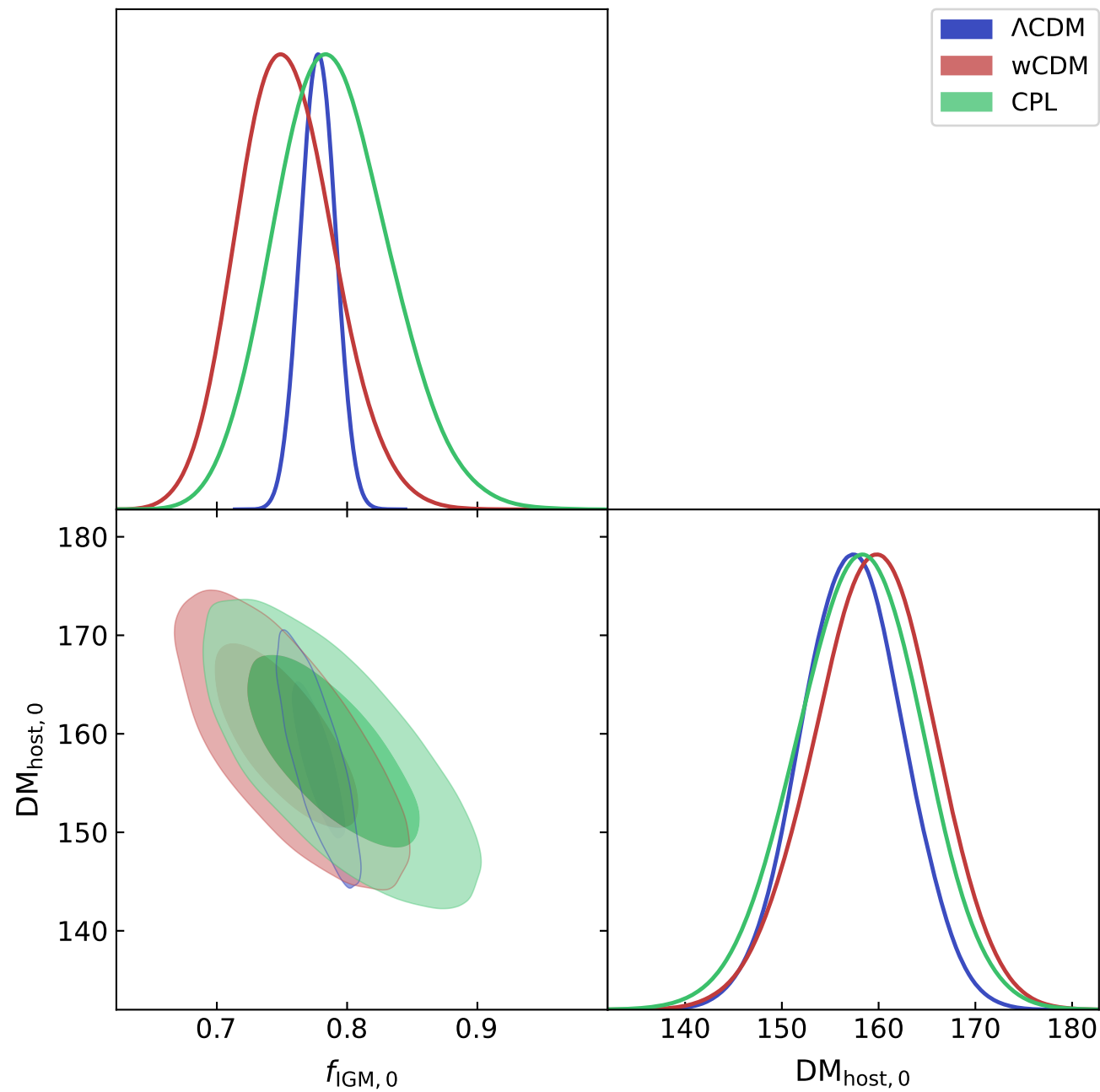
Case A — Constant f_{\text{IGM}} : cosmological model comparison
