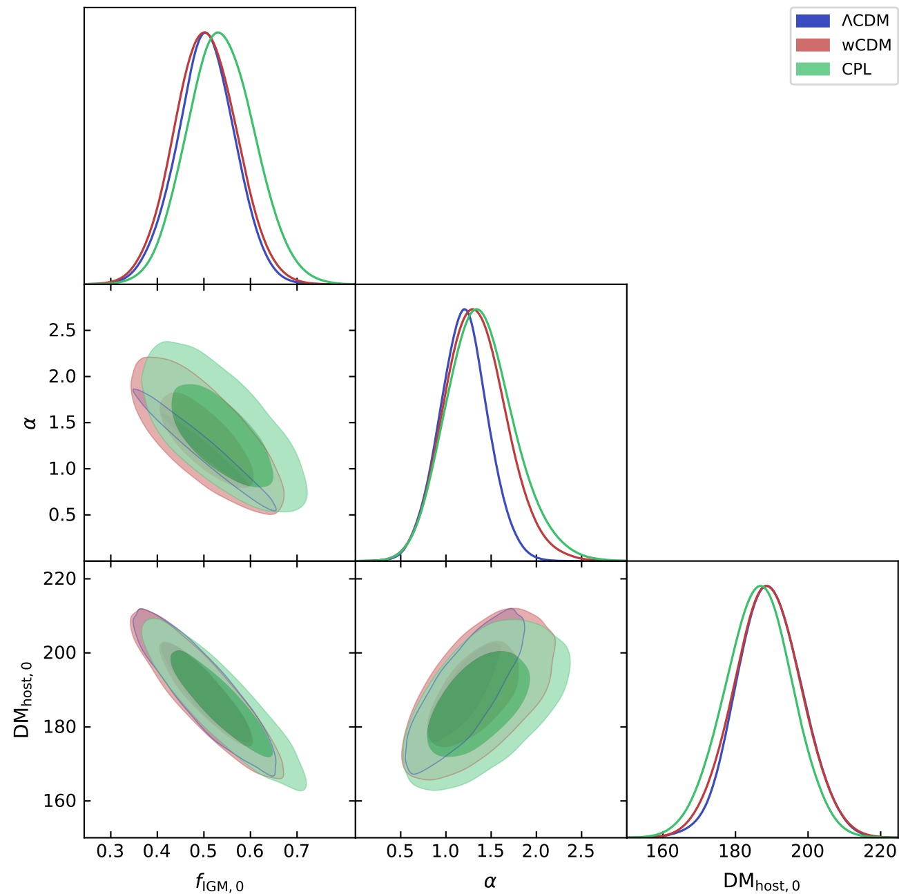
Case B — Time-dependent f_{\text{IGM}} : cosmological model comparison
