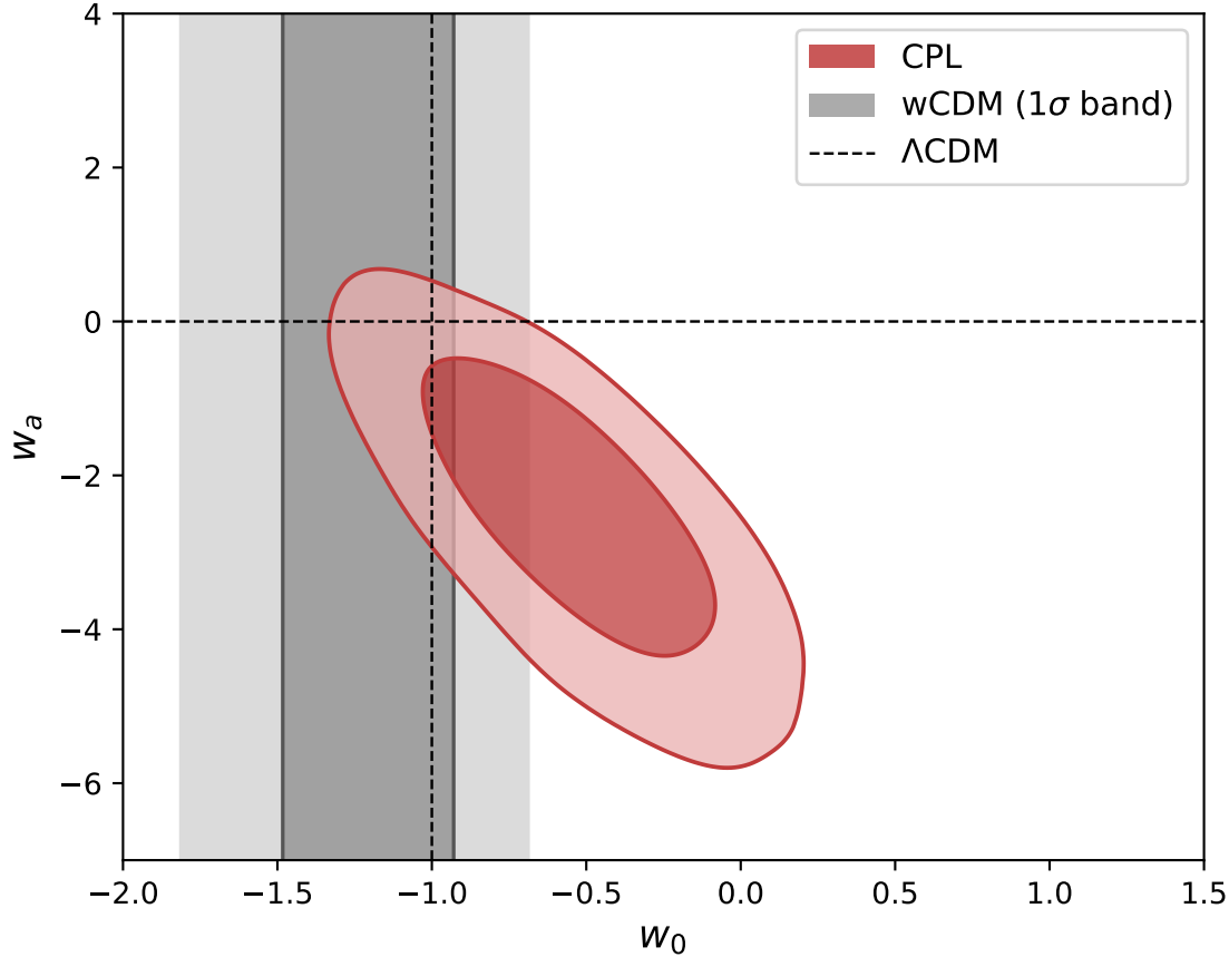
Case A — Constant f_{\text{IGM}}
