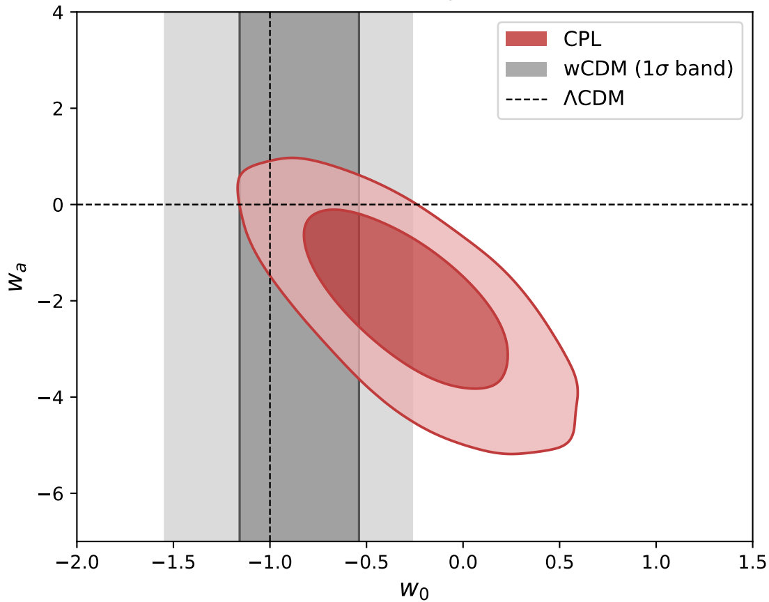
Case B — Time-dependent f_{\text{IGM}}
