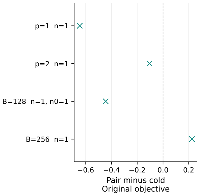
Cubic spin glass
