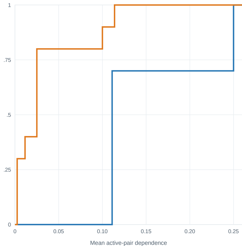
Mean active-pair dependence
