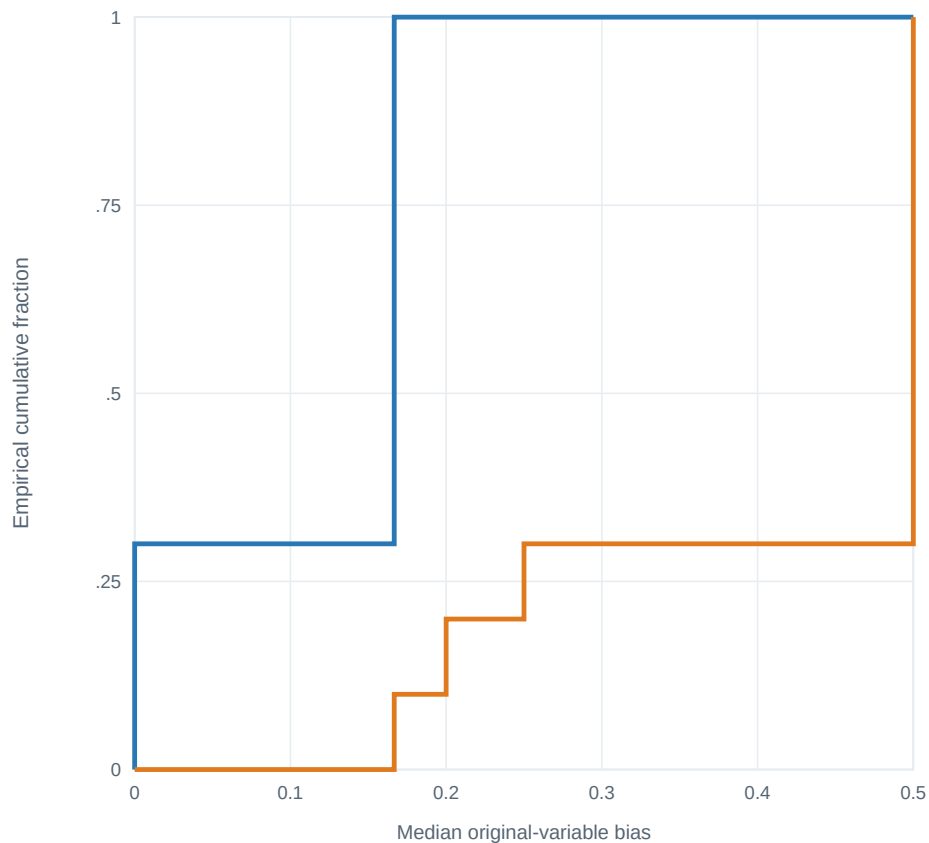
Median original-variable bias
