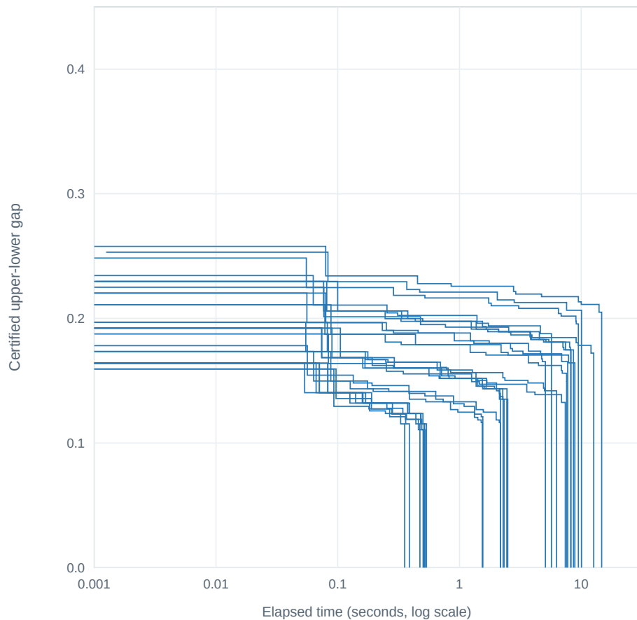
Cubic spin glass (N=30)
