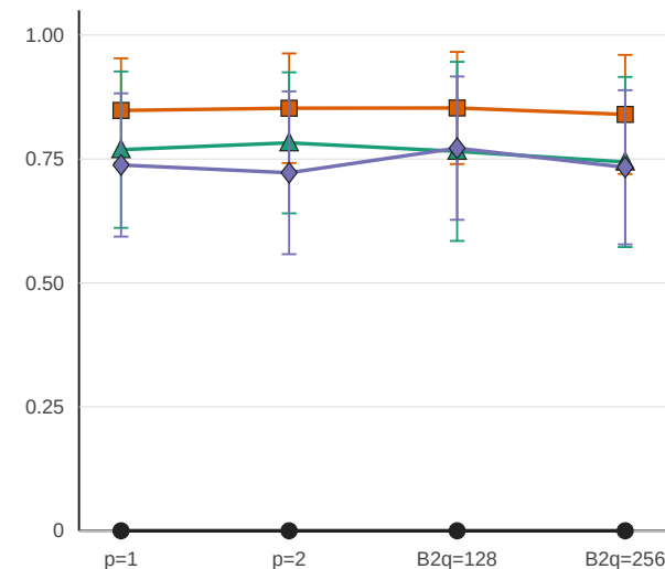
Max-3SAT: Auxiliary inconsistency, R_inc
