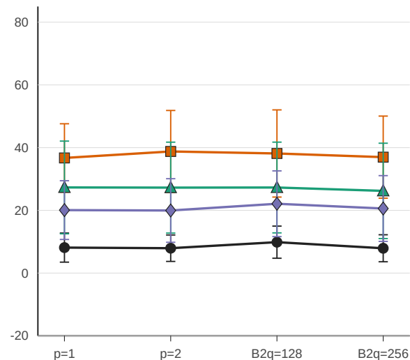
Max-3SAT: Mean encoded energy
