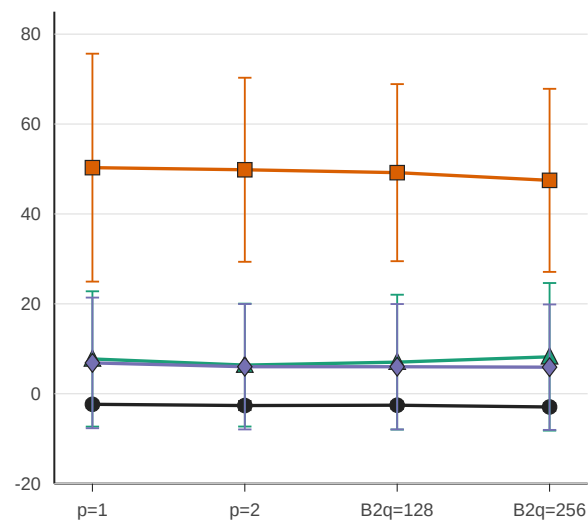
Cubic spin glass: Mean encoded energy
