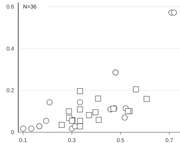
All-to-all: Routing overhead
