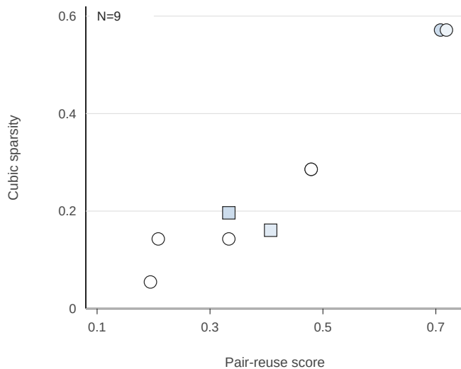
12-qubit 3 x 4 grid: Two-qubit gates
