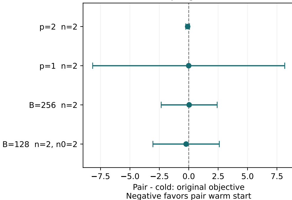
Spin glass
