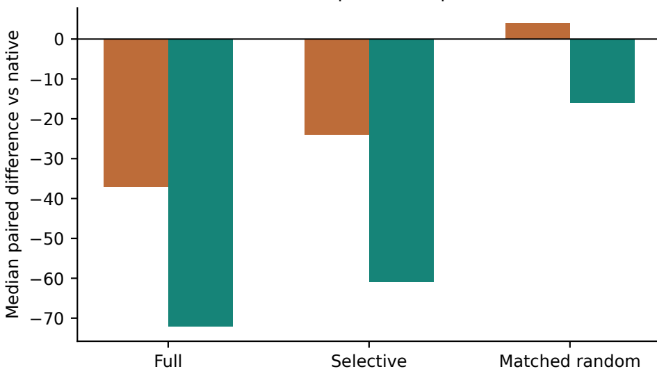
Max-3SAT | All-to-all | n=90
